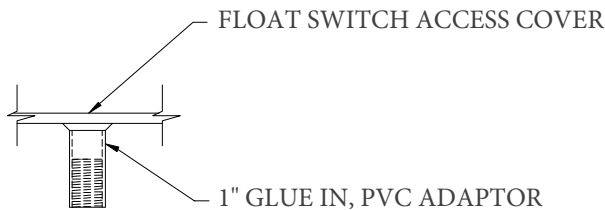
* GLUE IN, PVC ADAPTOR DETAIL
